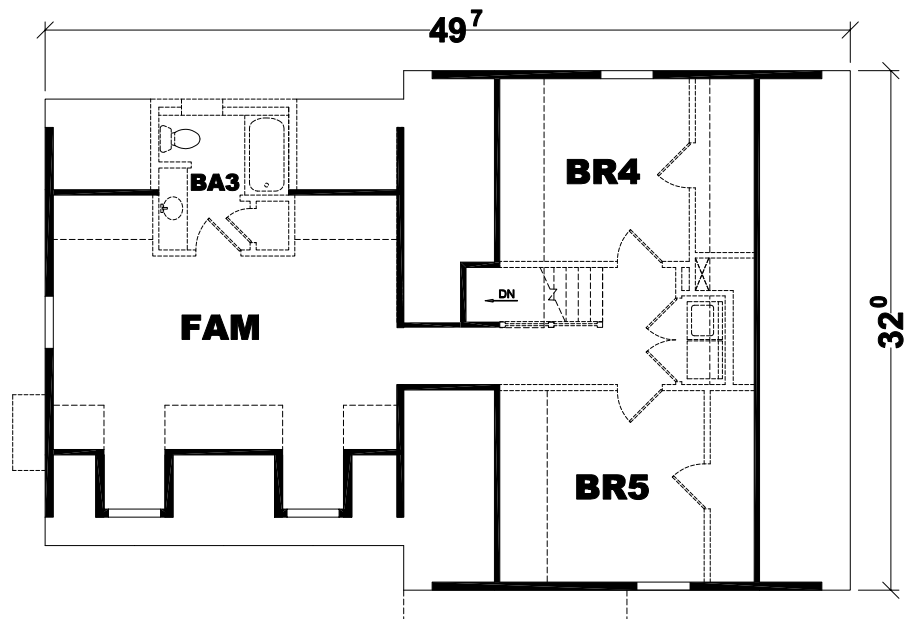
Proposed Second Floor Layout
